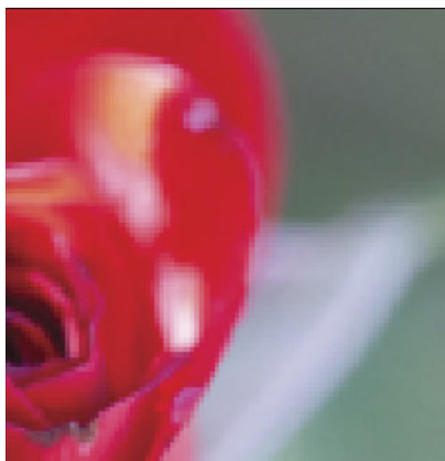
Nearest Neighbor
