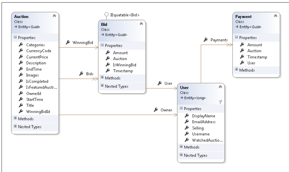
Figure 8-2. Domain model
