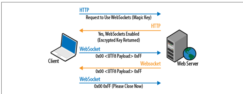
Figure 11-4. WebSockets
