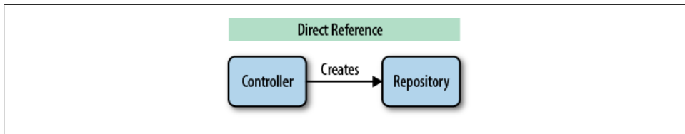
Figure 5-6. Managing dependencies
