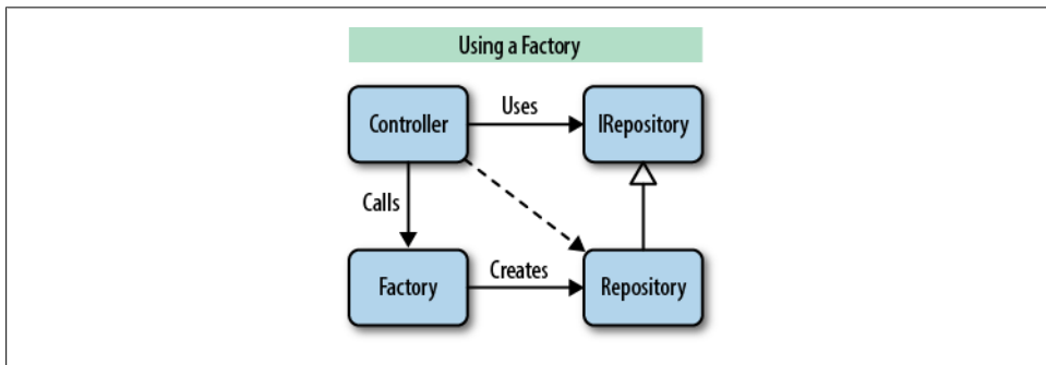
Figure 5-7. Using abstraction
