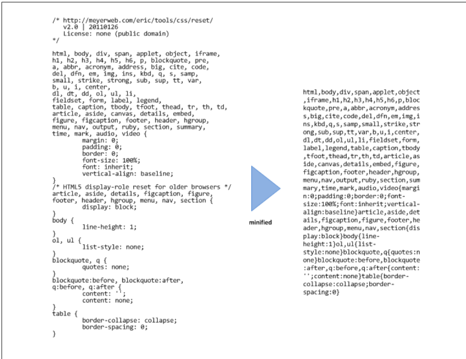
Figure 13-8. Minifying scripts and styles improves response times
