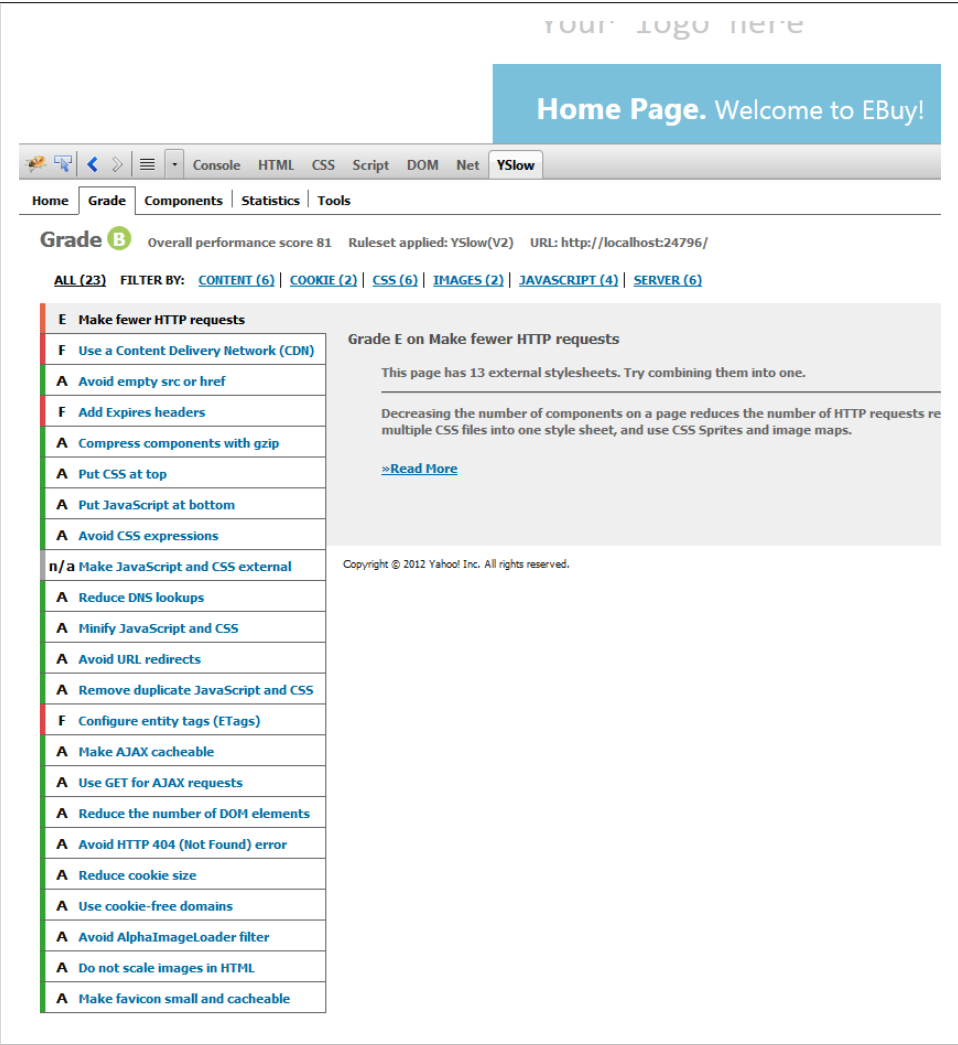
Figure 13-12. The starter template scores pretty well on its own!
