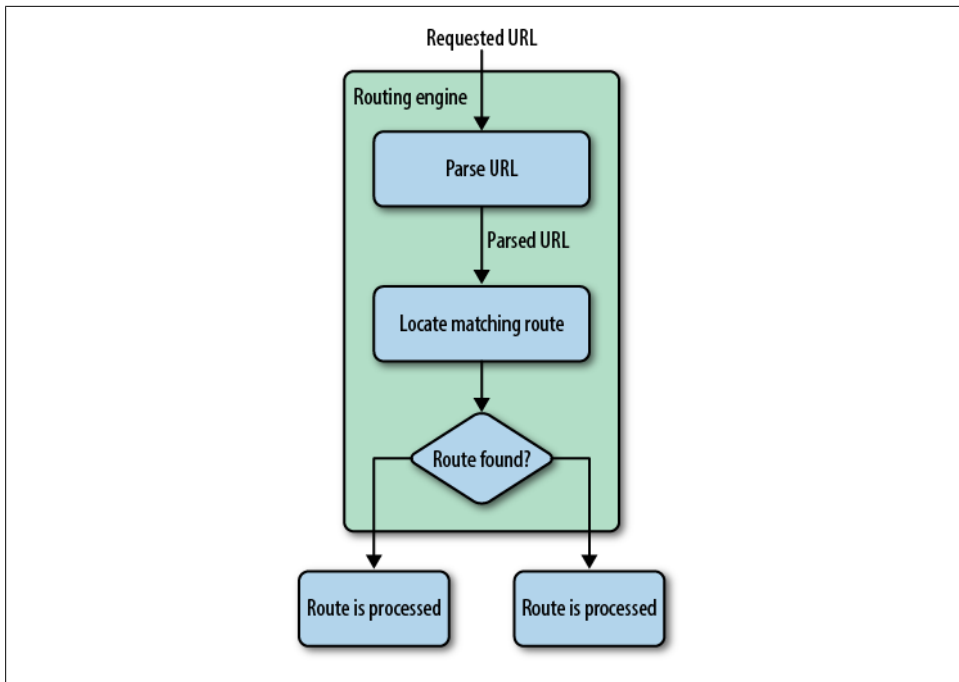
Figure 1-6. ASP.NET routing
