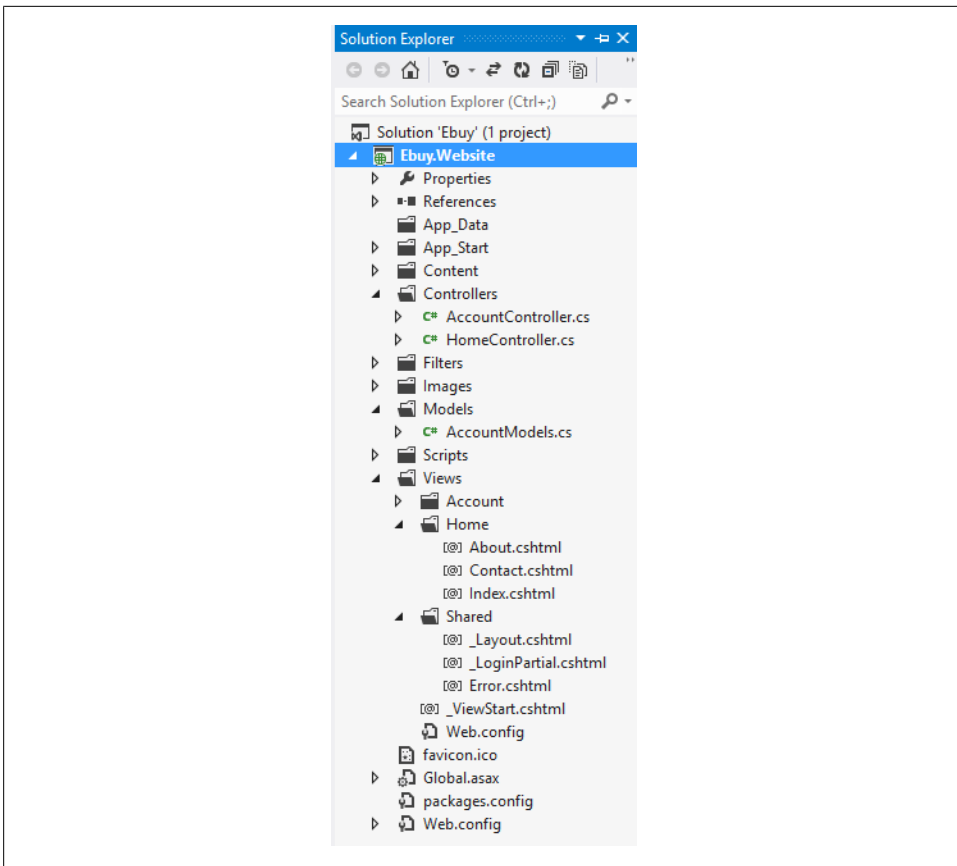
Figure 1-4. The ASP.NET MVC project folder structure
